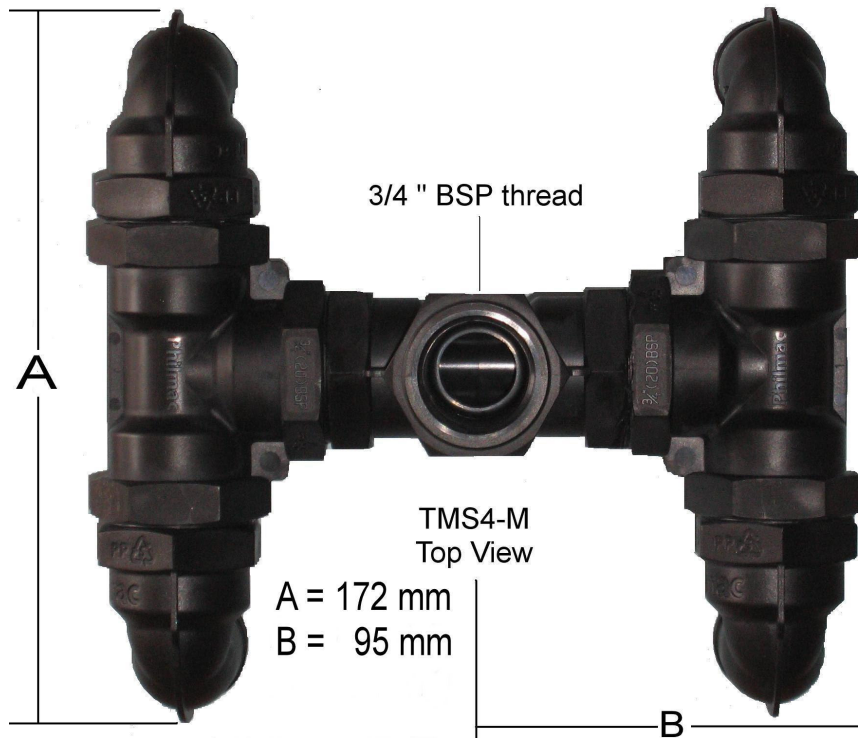
TMS4-M 4 Way Manifold Heat welded polypropylene
