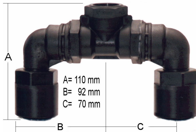
TMS2-M 2-Way Manifold Heat Welded Polypropylene
